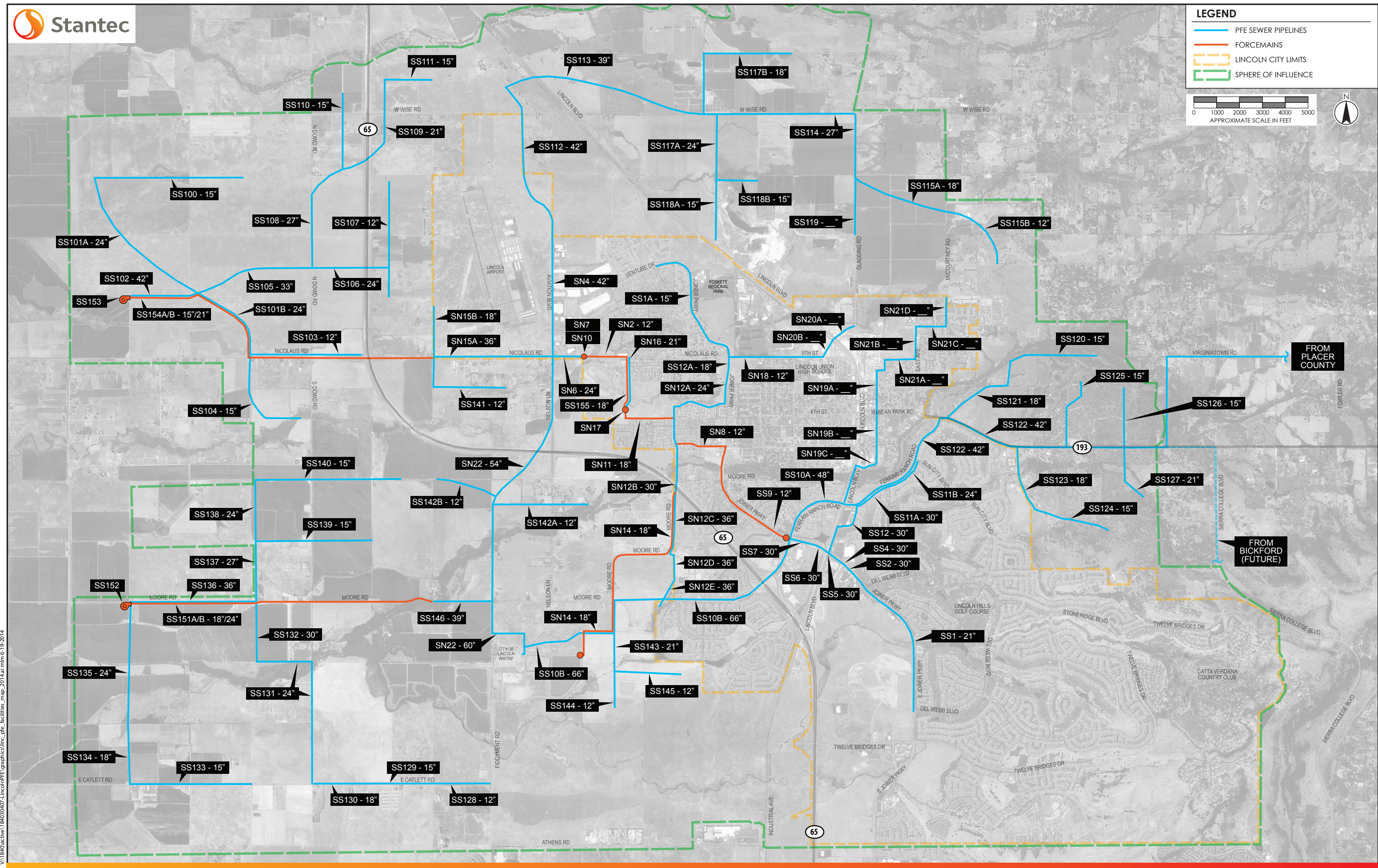
Figure 1 City of Lincoln 2014 PFE Update - Wastewater Facilities Map
